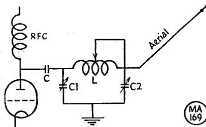
Fig. 2. The pi-section coupler, allowing almost any length of direct-on wire to be resonated at any frequency, within wide limits. This arrangement is specially useful for HF aerials when operated off their true mode on the LF bands.
