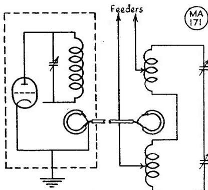
Fig. 4. Link coupled aerial tuning system, typical of many well designed amateur installations. Its advantages are discussed in the text.
