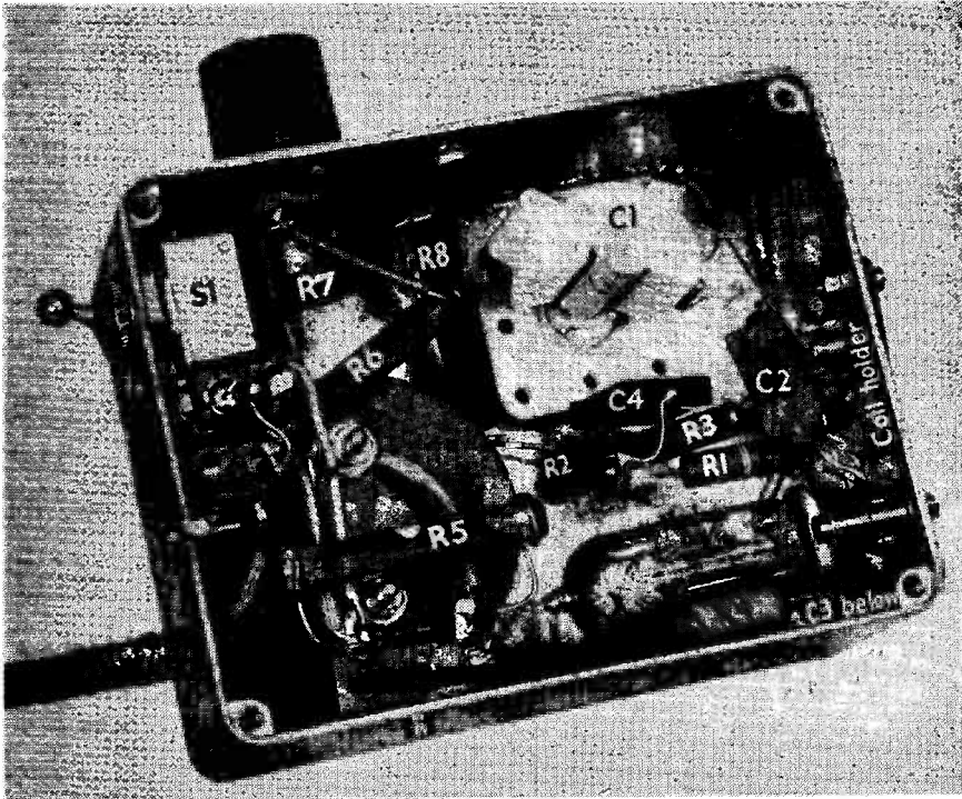
Showing the construction inside the Grid Dip Oscillator unit described by G5JU, with major components identified.
