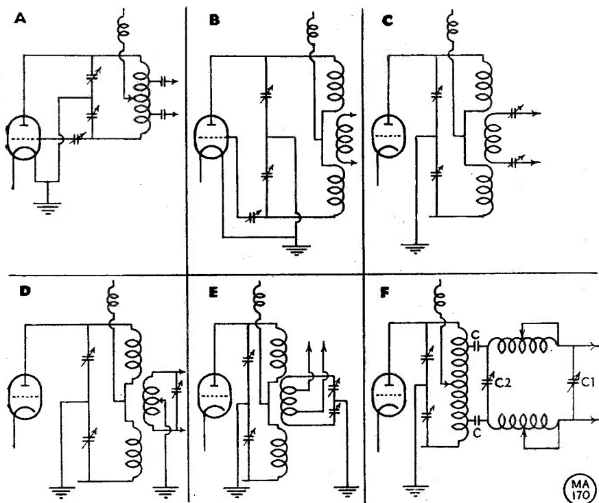
Fig. 3. A variety of coupling methods when using twin open-wire feeder to energise the aerial.
