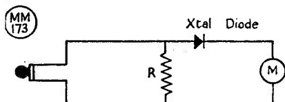
Fig. 2. The plug-in null indicator, discussed in the text. The crystal diode can be a 1N21 or 1N34, the meter 0-1 mA or 0-500 \mu A, and the value of R is a matter of experiment, 8000 ohms being about right for an 0-1 mA meter.
