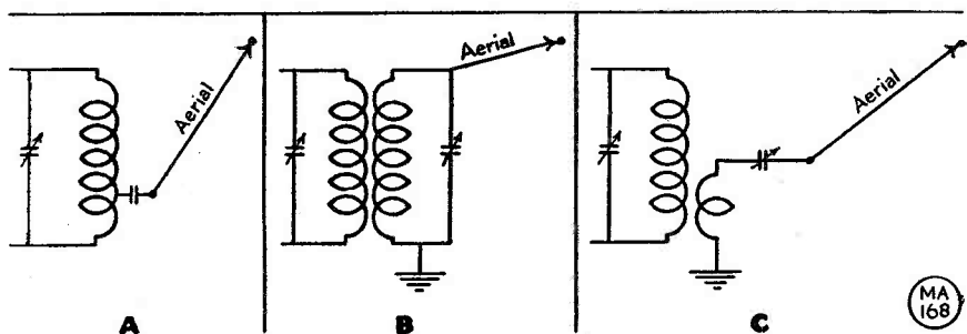
Fig. 1. Methods of exciting the aerial directly, discussed in detail in the text.
