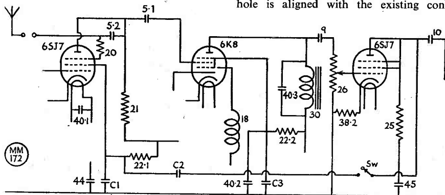
Fig. 1. Modifying the BC-221 as suggested by G2BVN. The numbers refer to components marked on the original BC-221 (T) circuit diagram. To carry out the modification the additional items required are: C1, .002 \mu F, mica; C2, C3, .01 \mu F mica; SPST toggle switch.
