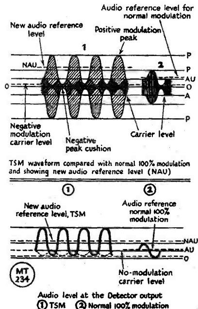
Fig. 2. Waveform diagrams to illustrate the discussion in the text.
