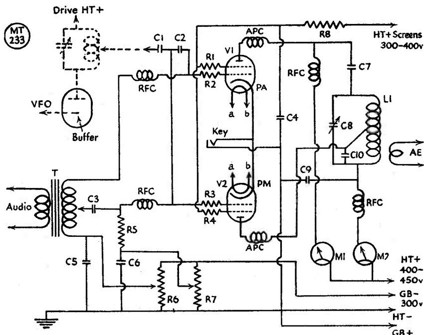
Fig. 1. Circuit of the PA/PM section of the 160-metre super modulated transmitter discussed by G2BCX.
